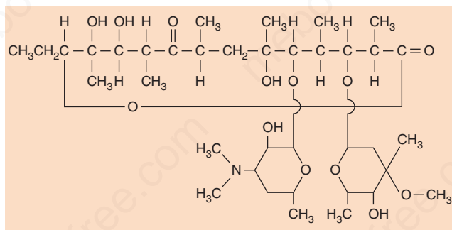
FIGURE 10-8 Erythromycin.
