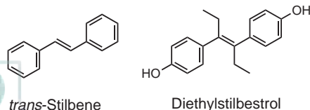
FIGURE 41.8 Nonsteroidal estrogens.
