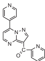
Ocinaflon
