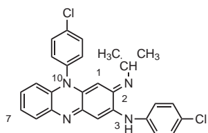
Clofazimine
