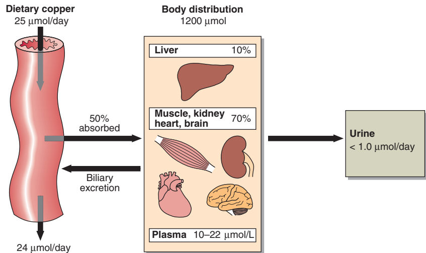
Fig 58.3 Copper balance.
