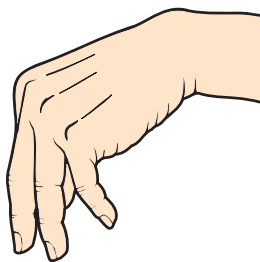
Fig 35.5 Trousseau's sign.
