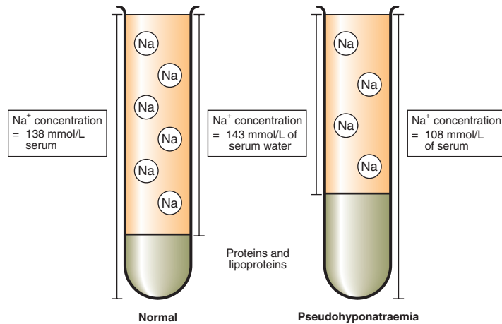
Fig 8.3 Pseudohyponatraemia.
